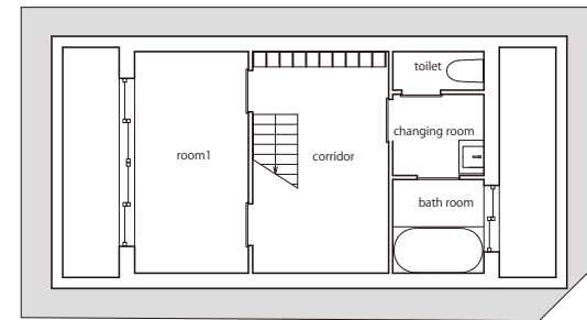
B1F Plan S=1/150
