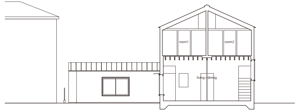
Section S=1/150
